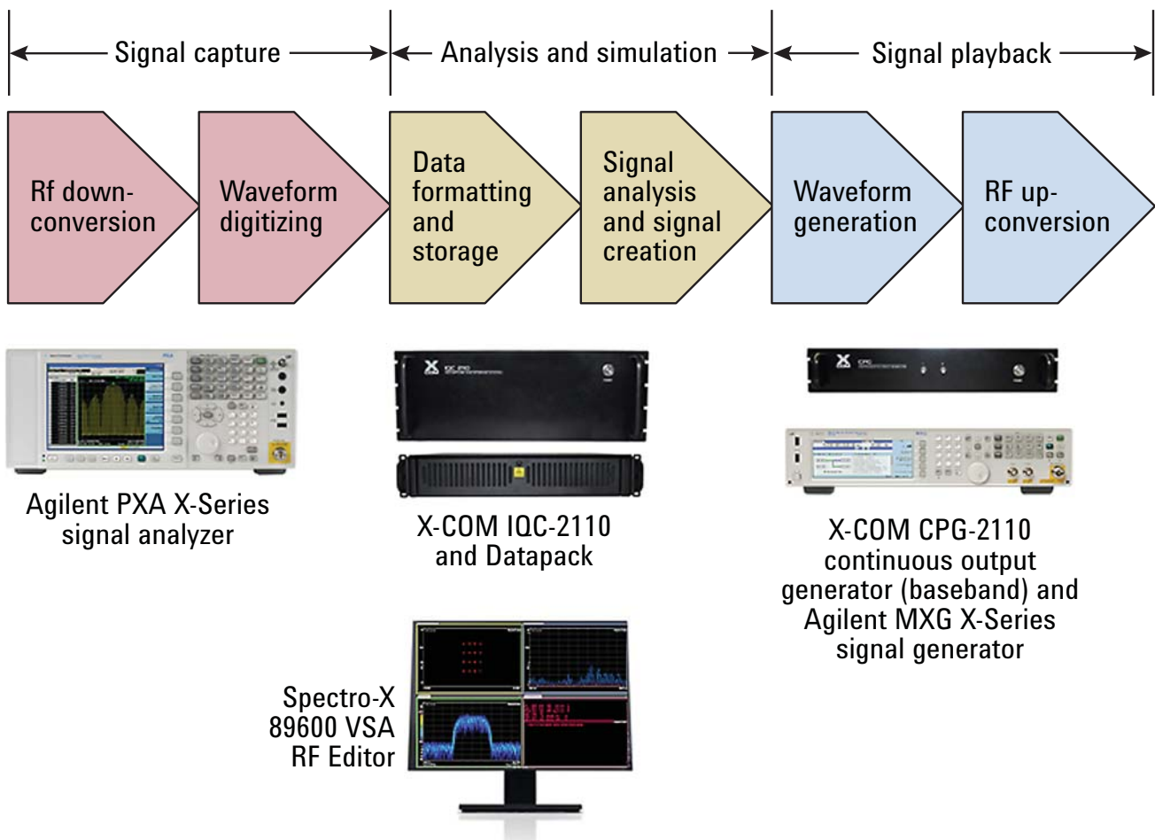
Figure 2. A combination of COTS hardware and software elements enables high-fidelity capture, analysis, simulation and playback
